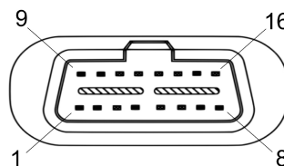
Figure 3: OBDII Connector
