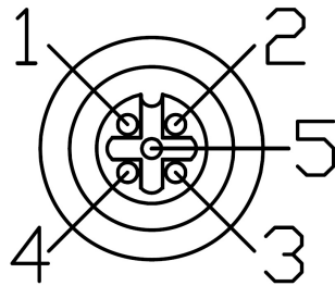
Figure 4: NMEA Connector
