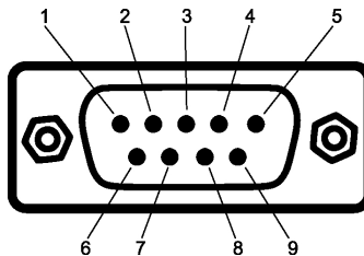
Figure 2: The D-SUB connector pin numbers
