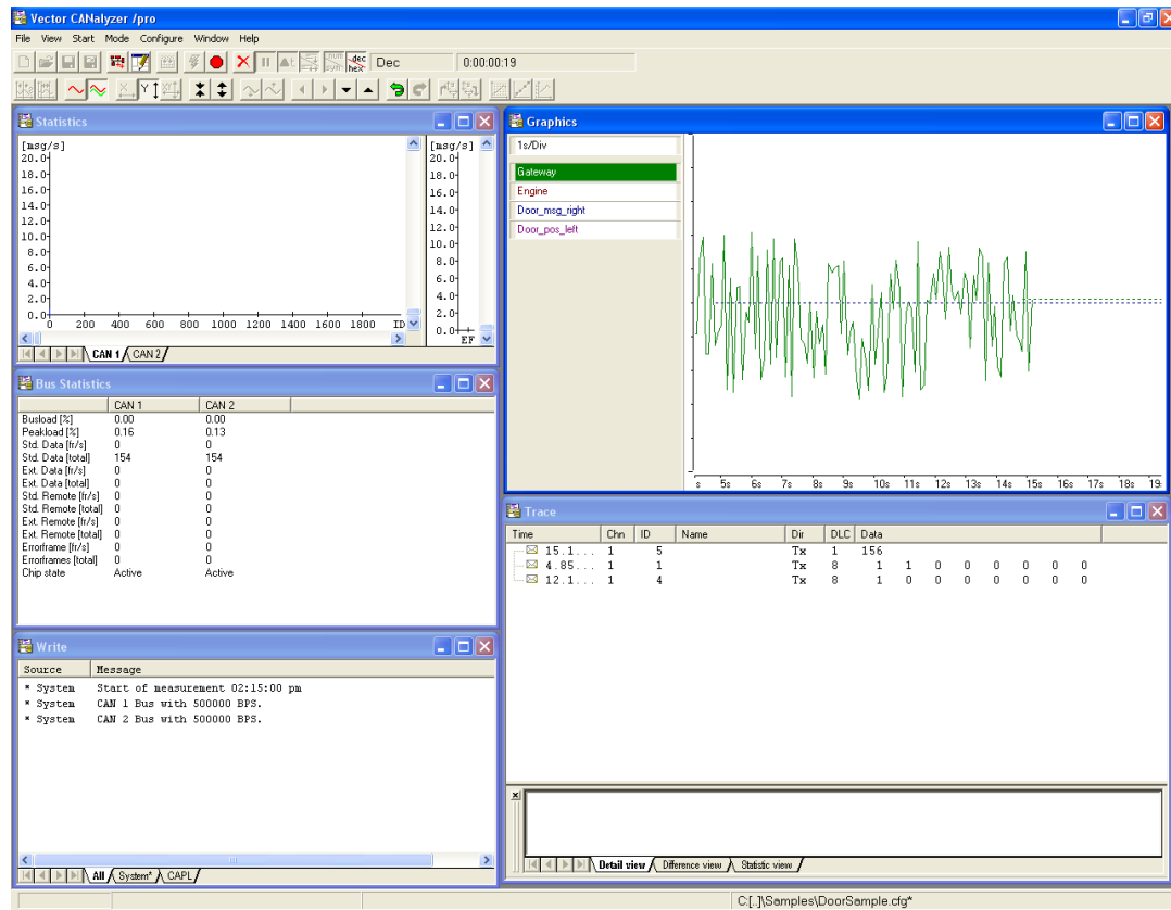
Figure 32. Replay in CANalyzer.
