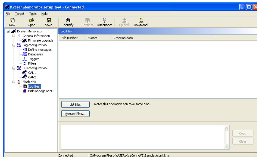
Figure 20. Log files.
