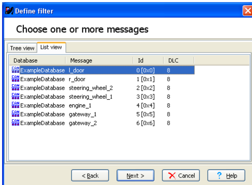
Figure 15. Choose message.
