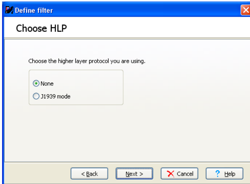
Figure 14. Choose HLP.
