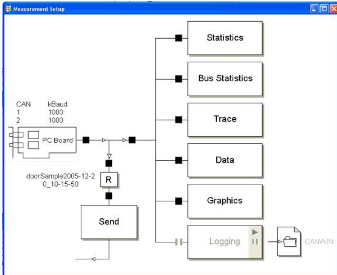
Figure 28. Measurement setup.
