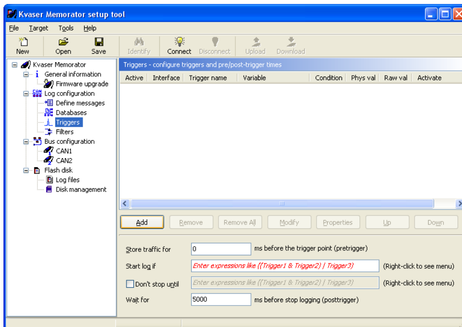
Figure 4 Triggers.
