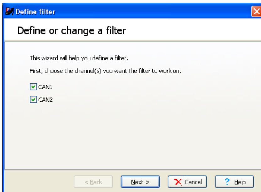
Figure 13. Define filter.
