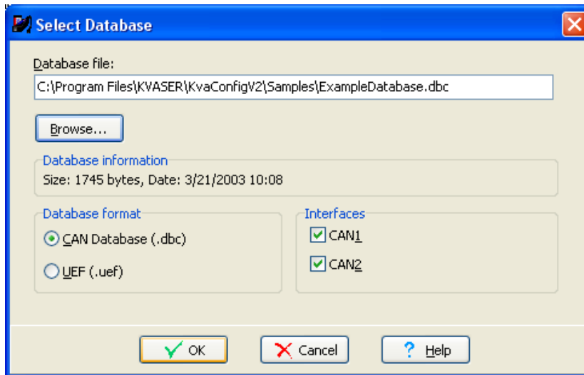
Figure 2. Add Database.
