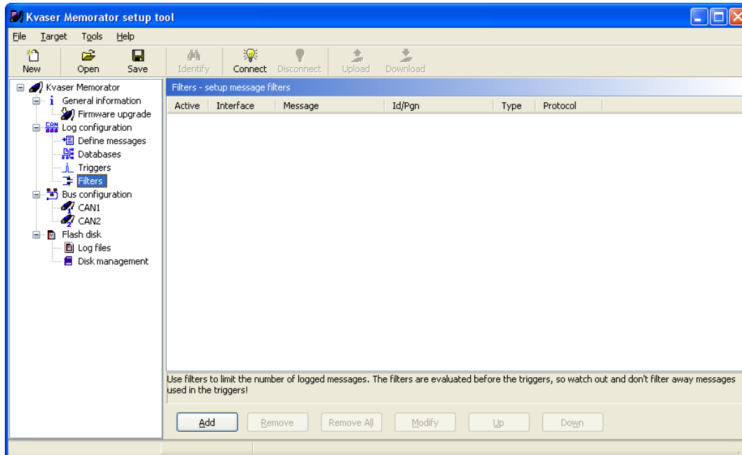
Figure 12. Filters.
