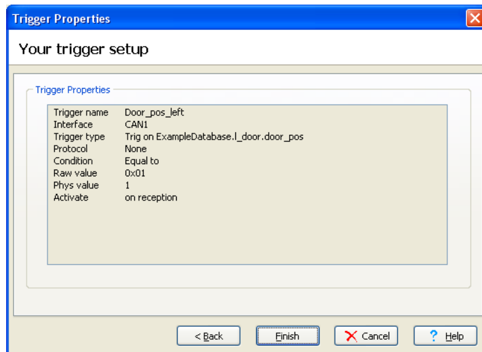
Figure 9. Trigger setup.
