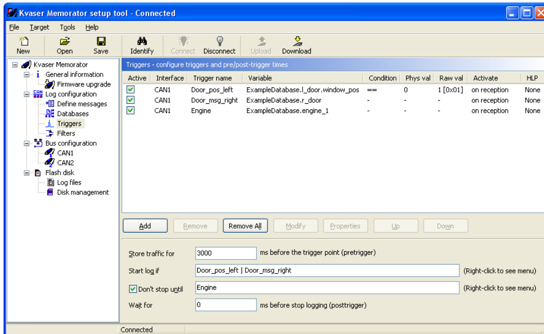
Figure 11. Trigger settings.
