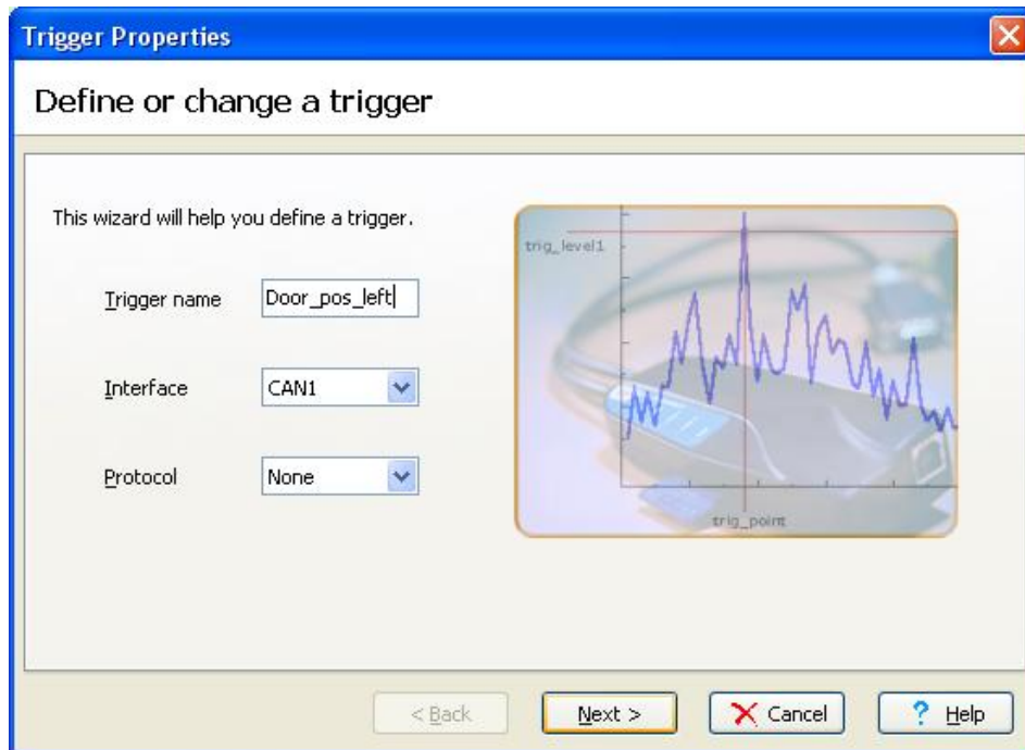
Figure 5. Add trigger.
