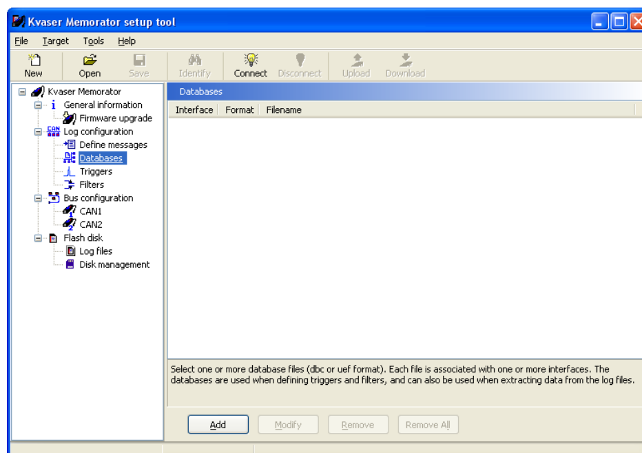
Figure 1. Databases.
