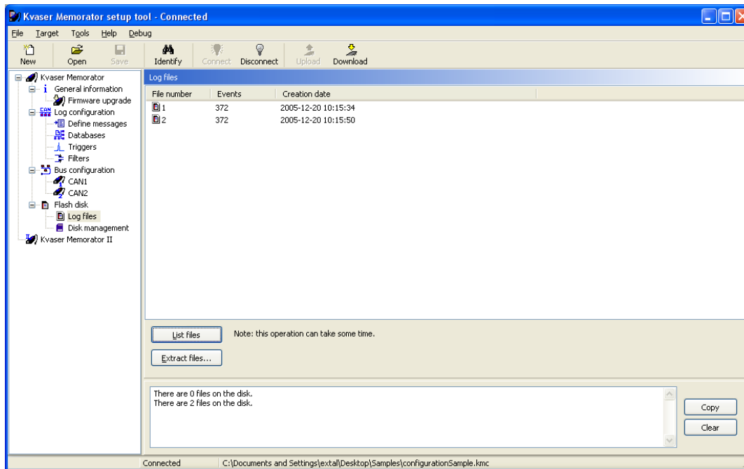
Figure 21. List files.
