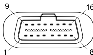
Figure 4: OBDII Connector
