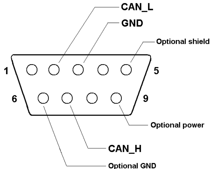
This is a male connector viewed from the connector side, or a female connector viewed from the soldering side.
